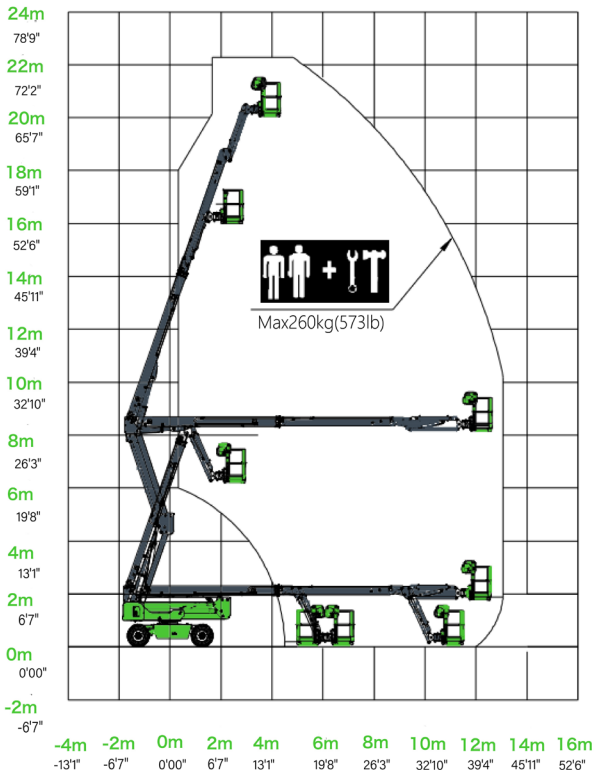
LA20JE Working Range
